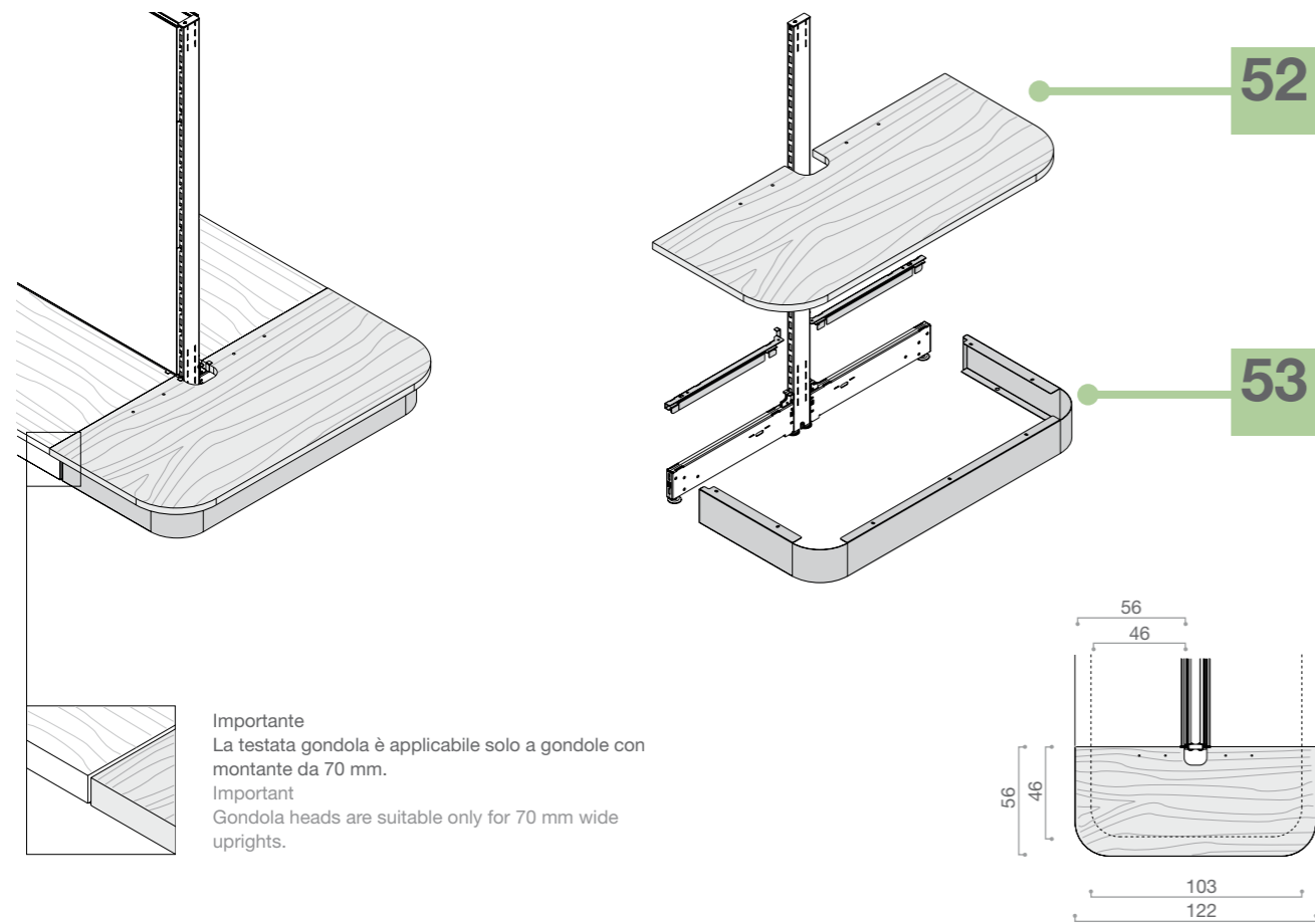
52 Ripiano base testata gondola Gondola head base shelf
